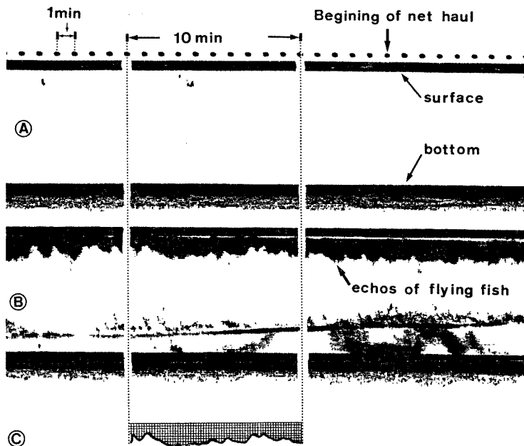
Fig. 2. An example of the Tele-sounder records. (A): Record by transducer A, (B): Record by transducer B, (C): Measurement of the Tele-sounder record as indicated by square area of echo shown on the recording sheet (B).
